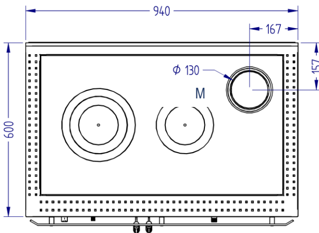
MODEL WITH UPPER FLUE GAS OUTLET
